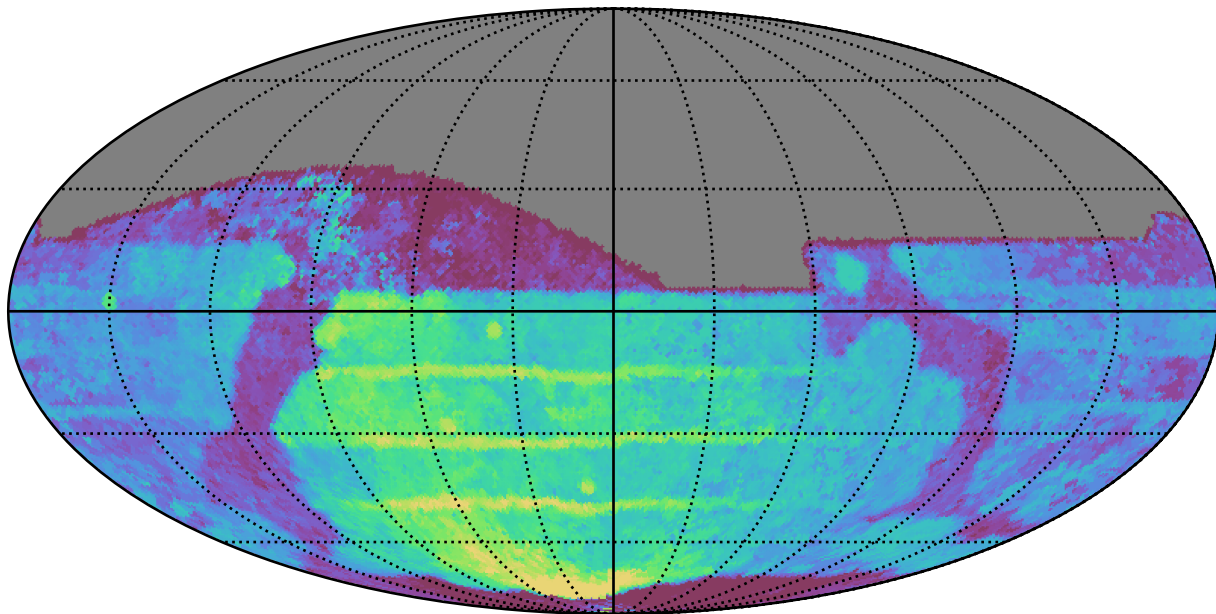
weather_cloudso16v3.4_10yrs All sky z band: Median Season Length
