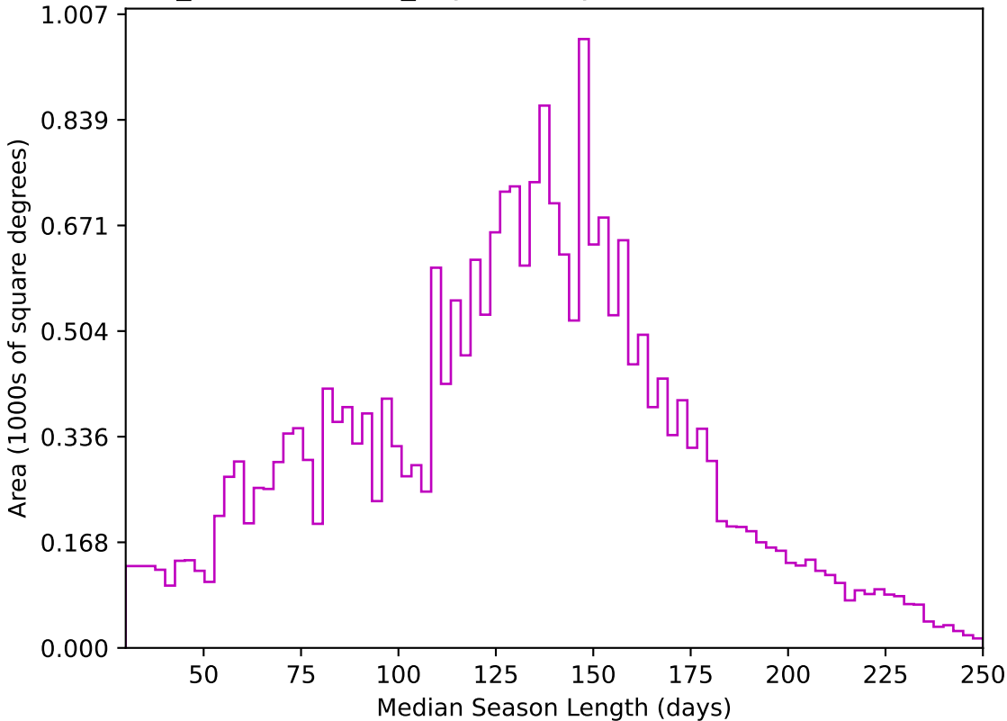
weather_cloudso16v3.4_10yrs All sky z band: Median Season Length
