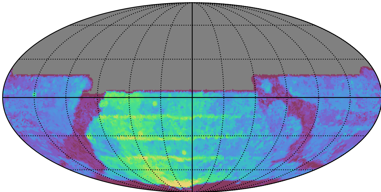
weather_cloudso16v3.4_10yrs All sky y band: Median Season Length
