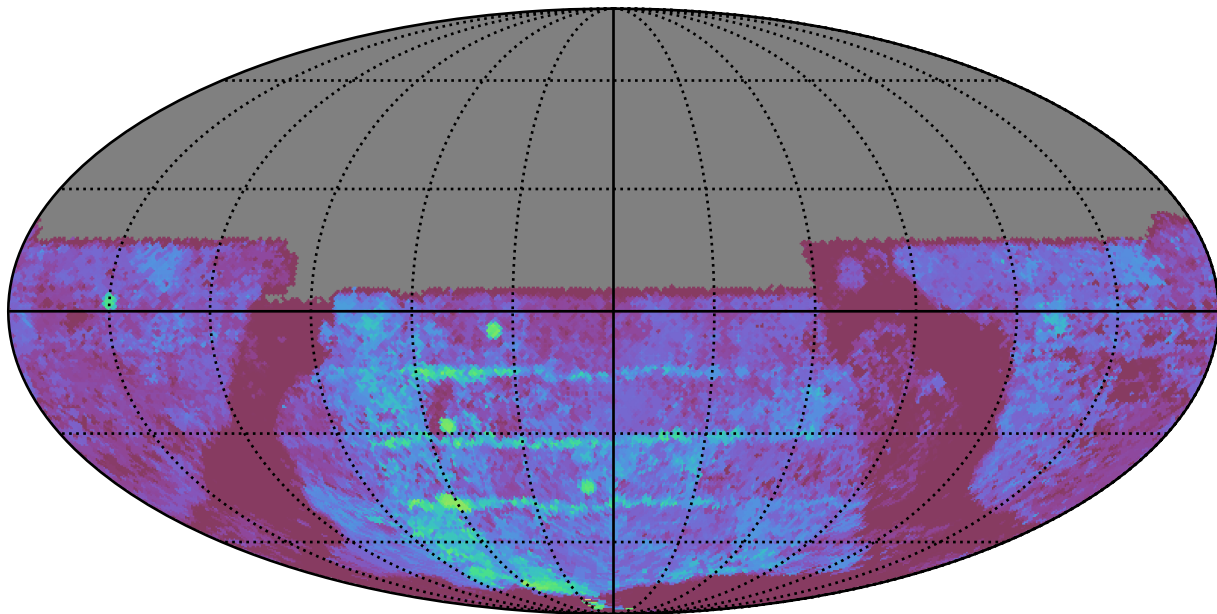
weather_cloudso16v3.4_10yrs All sky u band: Median Season Length
