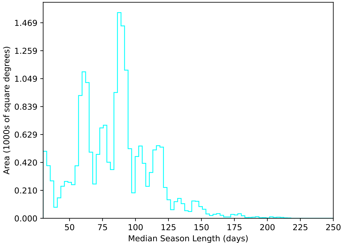
weather_cloudso16v3.4_10yrs All sky u band: Median Season Length
