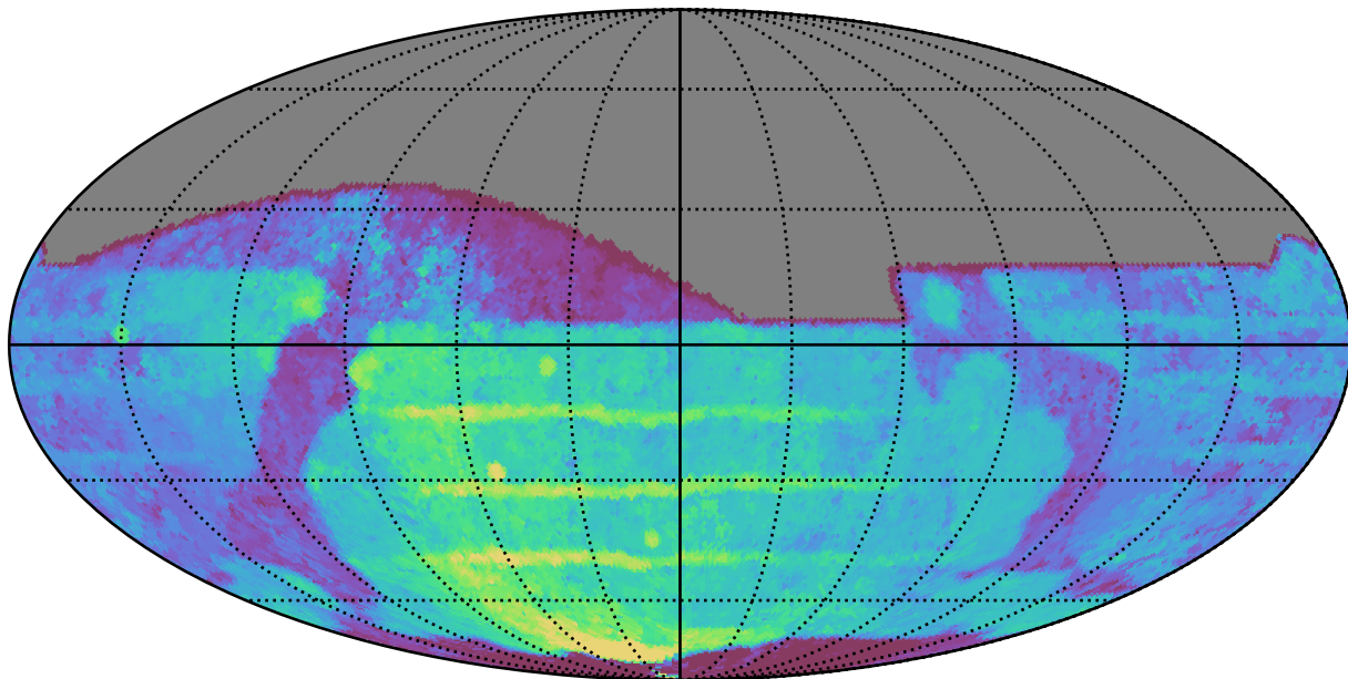
weather_cloudso16v3.4_10yrs All sky r band: Median Season Length
