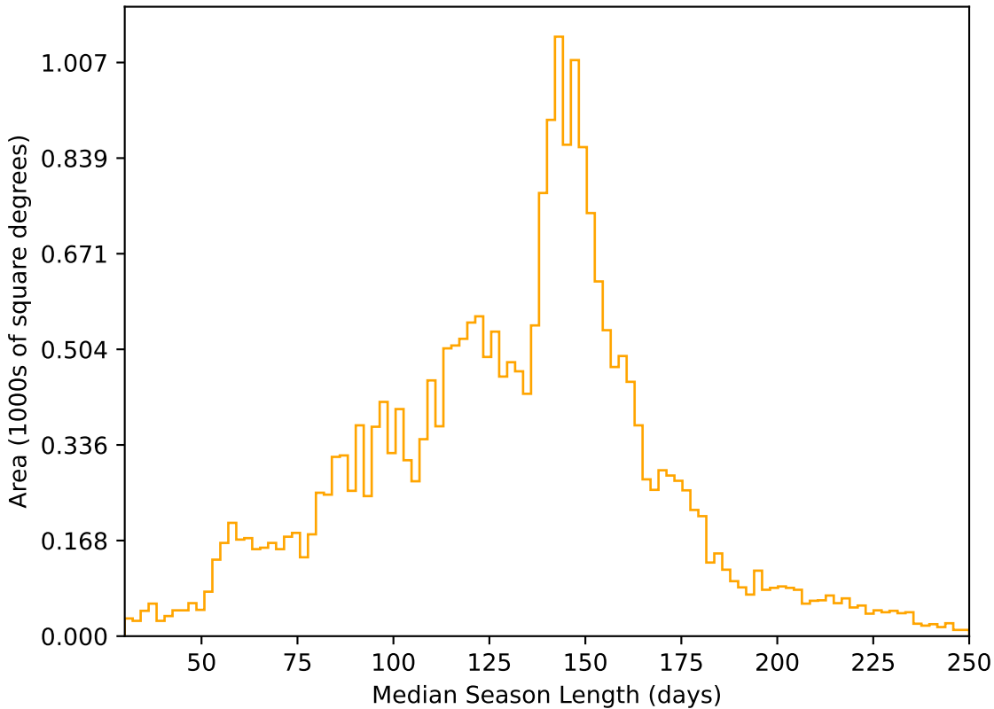
weather_cloudso16v3.4_10yrs All sky r band: Median Season Length
