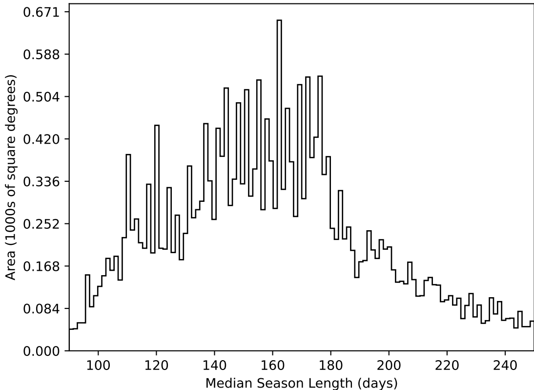
weather_cloudso16v3.4_10yrs All sky all bands: Median Season Length
