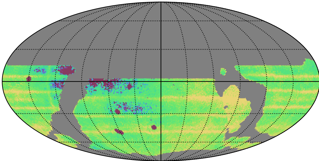
weather_cloudso16v3.4_10yrs WFD: Median Intra-Night Gap
