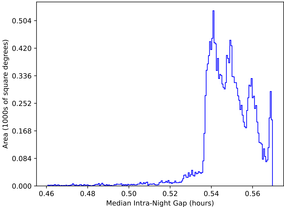
weather_cloudso16v3.4_10yrs WFD: Median Intra-Night Gap
