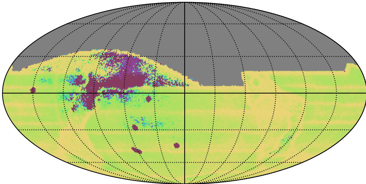
weather_cloudso16v3.4_10yrs All sky: Median Intra-Night Gap
