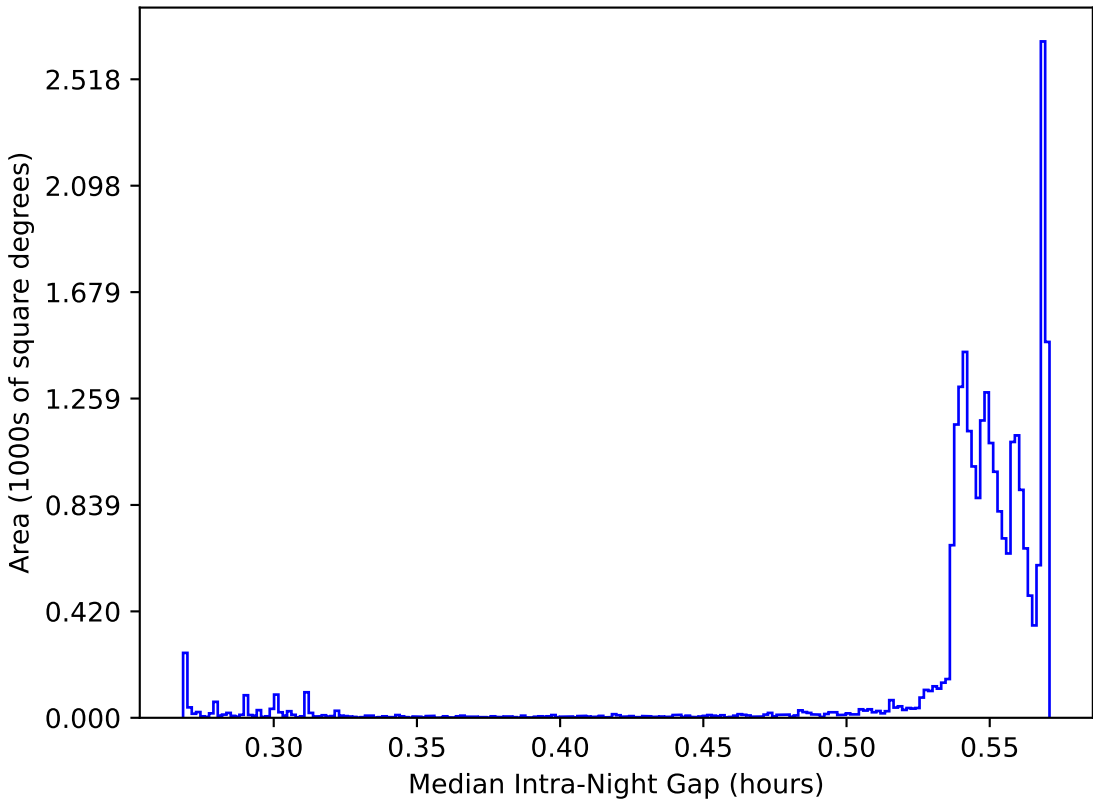
weather_cloudso16v3.4_10yrs All sky: Median Intra-Night Gap
