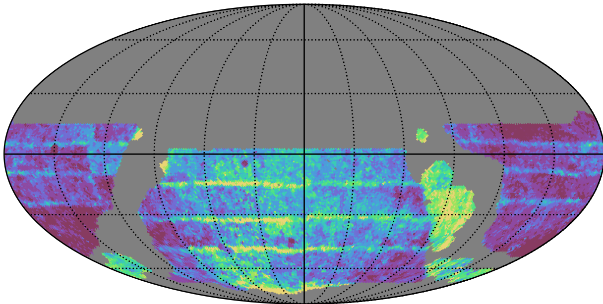
weather_cloudso16v3.4_10yrs WFD z band: Median Inter-Night Gap
