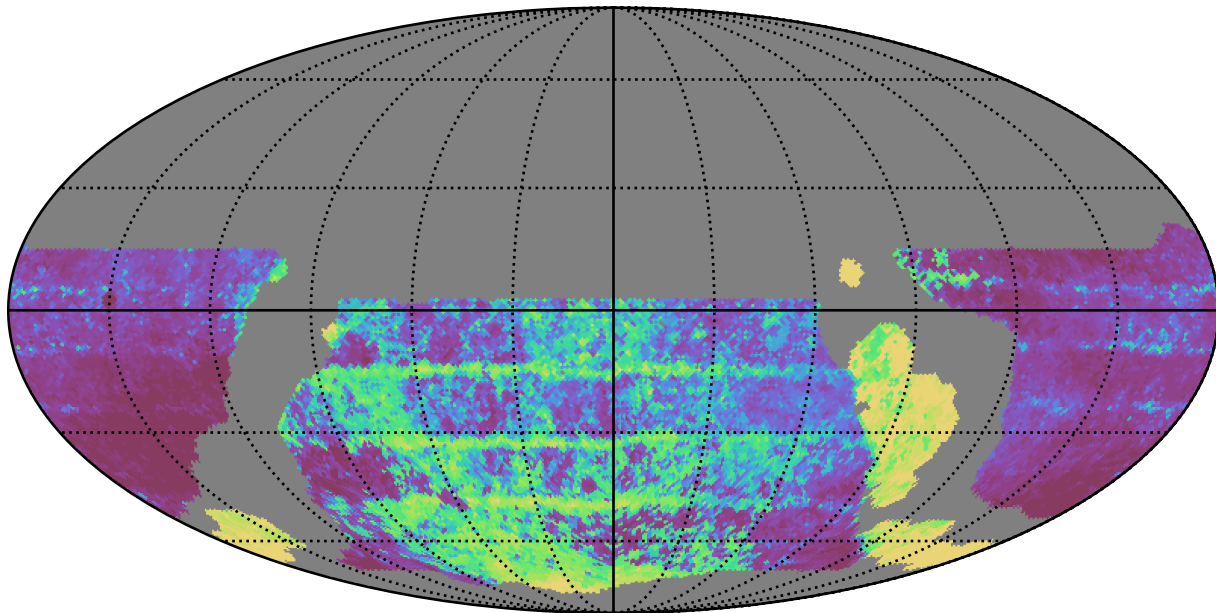
weather_cloudso16v3.4_10yrs WFD y band: Median Inter-Night Gap
