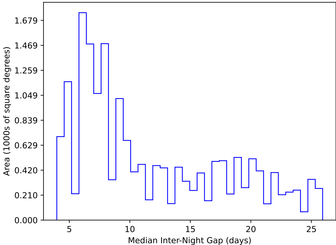
weather_cloudso16v3.4_10yrs WFD y band: Median Inter-Night Gap
