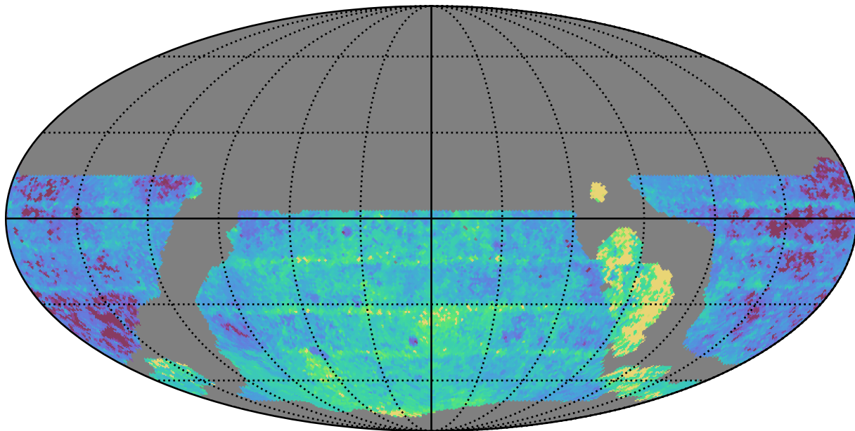
weather_cloudso16v3.4_10yrs WFD u band: Median Inter-Night Gap
