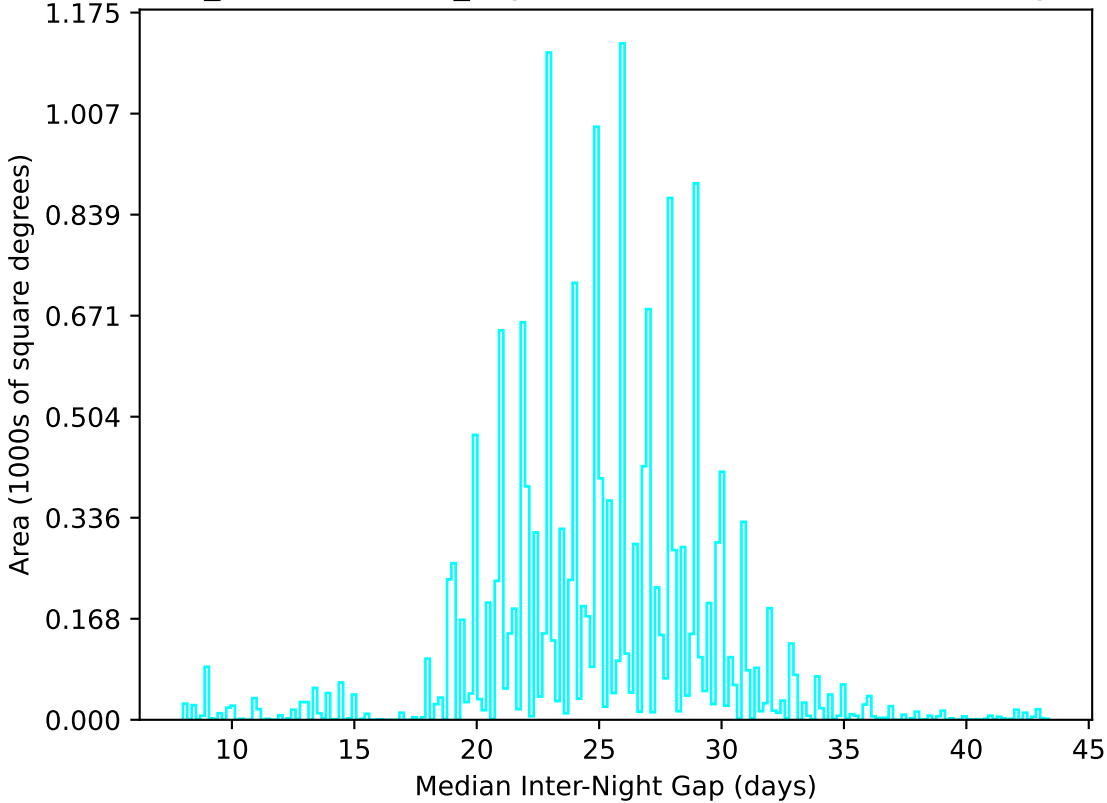
weather_cloudso16v3.4_10yrs WFD u band: Median Inter-Night Gap
