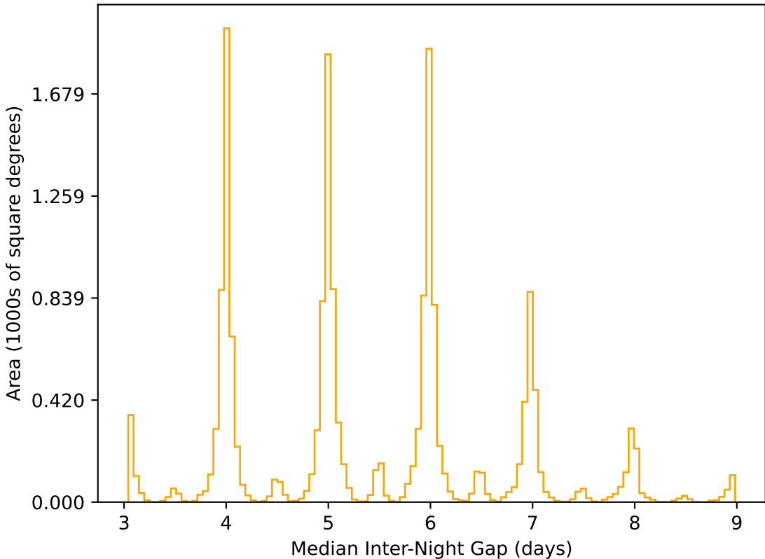
weather_cloudso16v3.4_10yrs WFD r band: Median Inter-Night Gap
