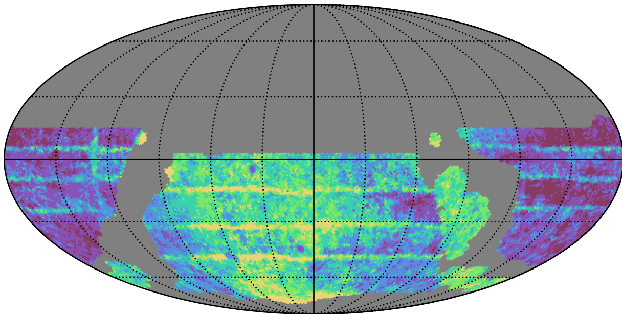
weather_cloudso16v3.4_10yrs WFD i band: Median Inter-Night Gap
