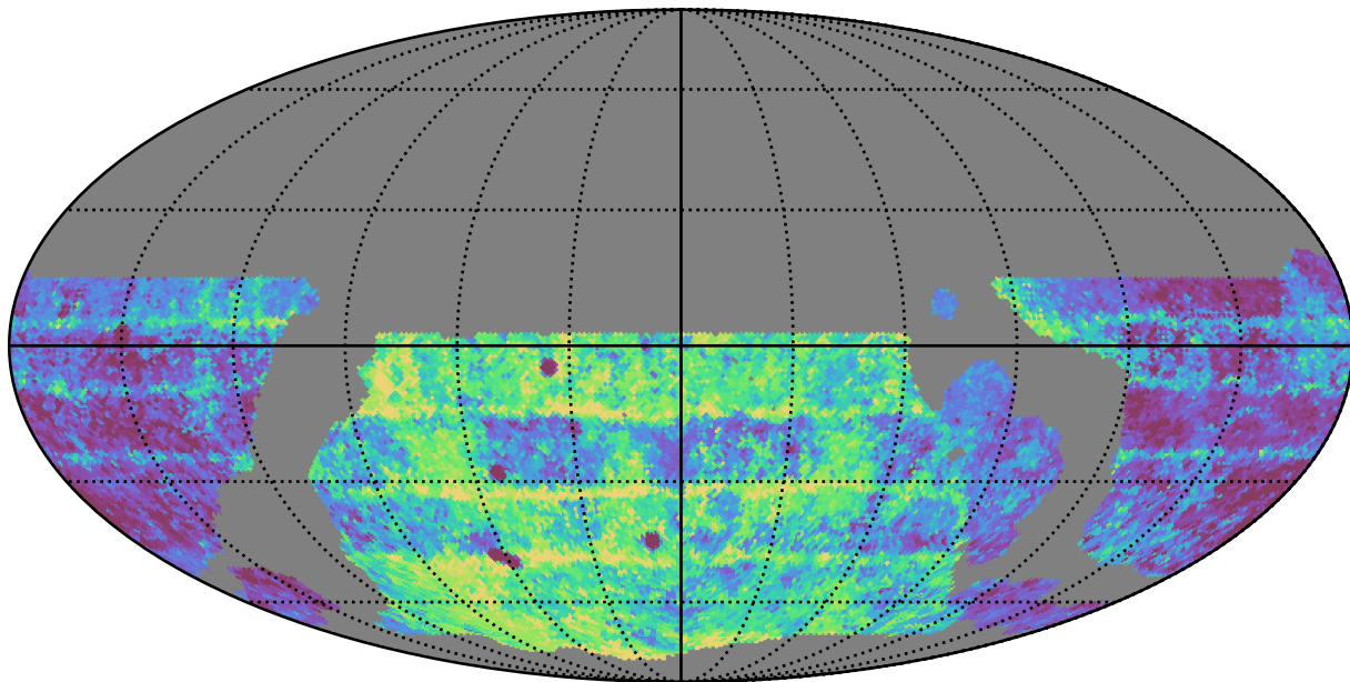
weather_cloudso16v3.4_10yrs WFD g band: Median Inter-Night Gap
