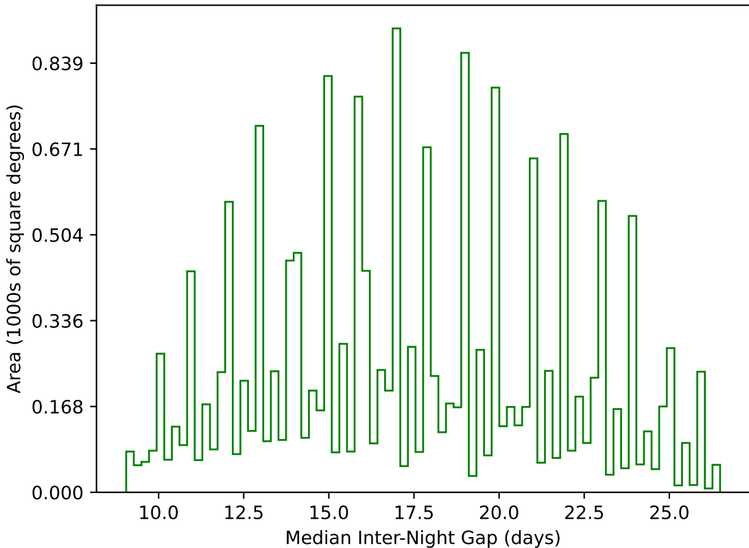
weather_cloudso16v3.4_10yrs WFD g band: Median Inter-Night Gap
