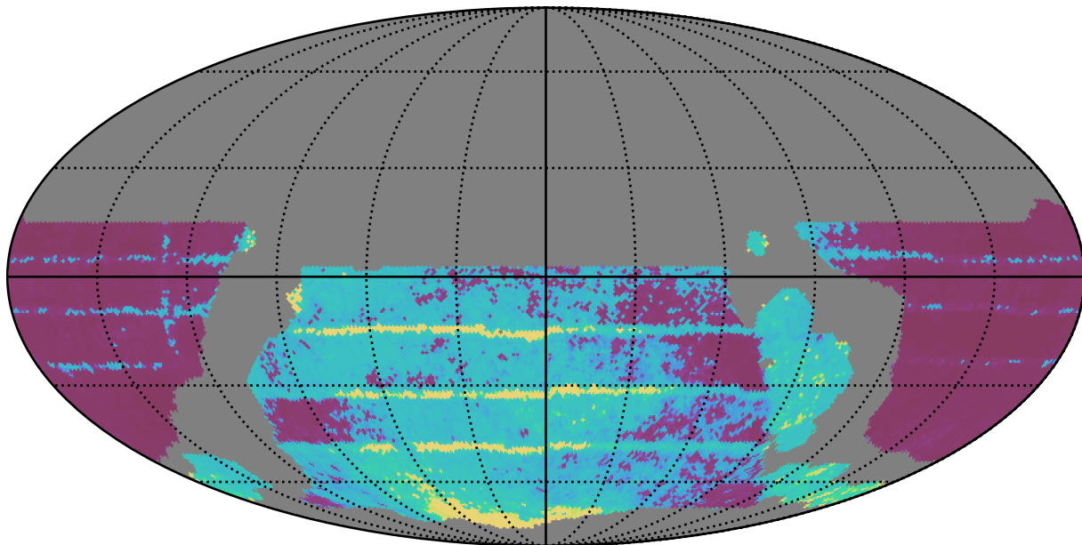
weather_cloudso16v3.4_10yrs WFD all bands: Median Inter-Night Gap
