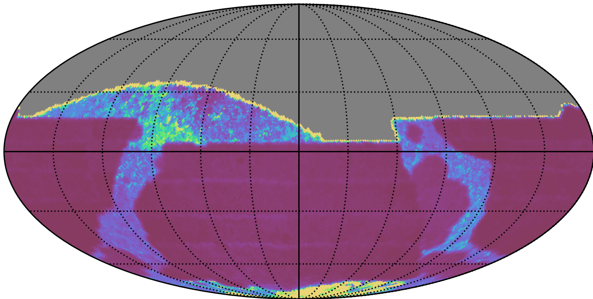
weather_cloudso16v3.4_10yrs All sky z band: Median Inter-Night Gap
