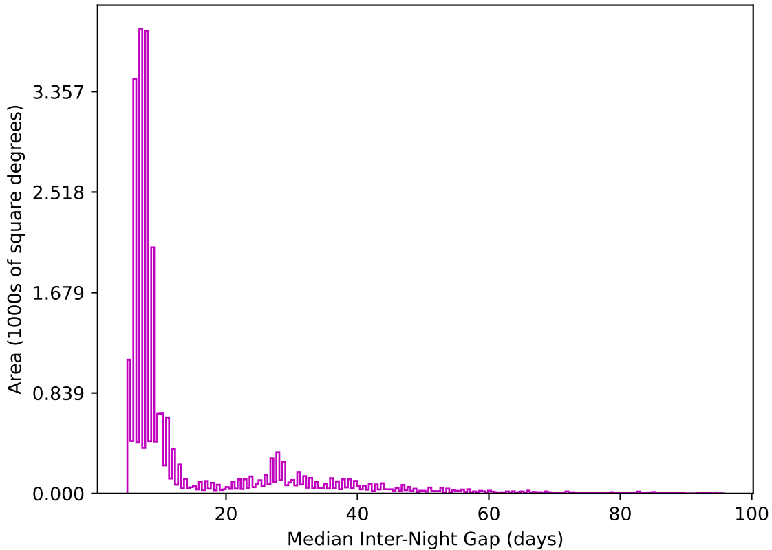
weather_cloudso16v3.4_10yrs All sky z band: Median Inter-Night Gap
