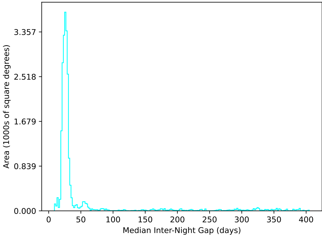
weather_cloudso16v3.4_10yrs All sky u band: Median Inter-Night Gap
