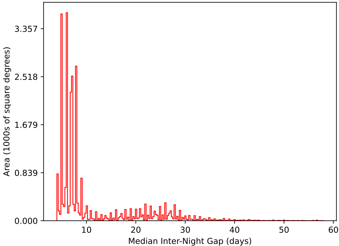
weather_cloudso16v3.4_10yrs All sky i band: Median Inter-Night Gap
