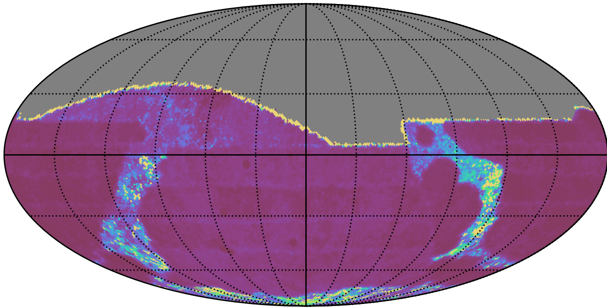
weather_cloudso16v3.4_10yrs All sky g band: Median Inter-Night Gap
