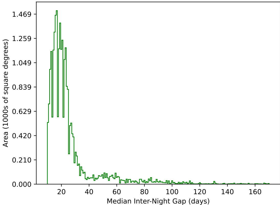
weather_cloudso16v3.4_10yrs All sky g band: Median Inter-Night Gap
