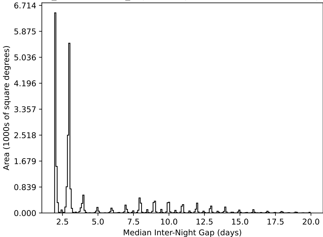
weather_cloudso16v3.4_10yrs All sky all bands: Median Inter-Night Gap
