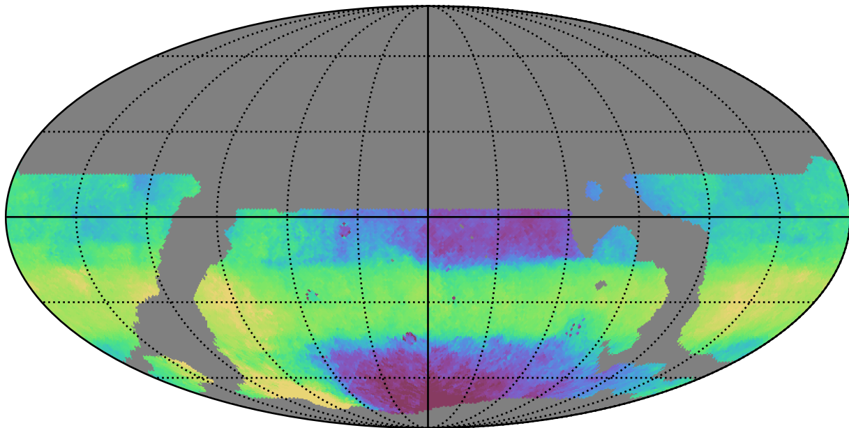
weather_cloudso16v3.4_10yrs WFD z band: Median HA
