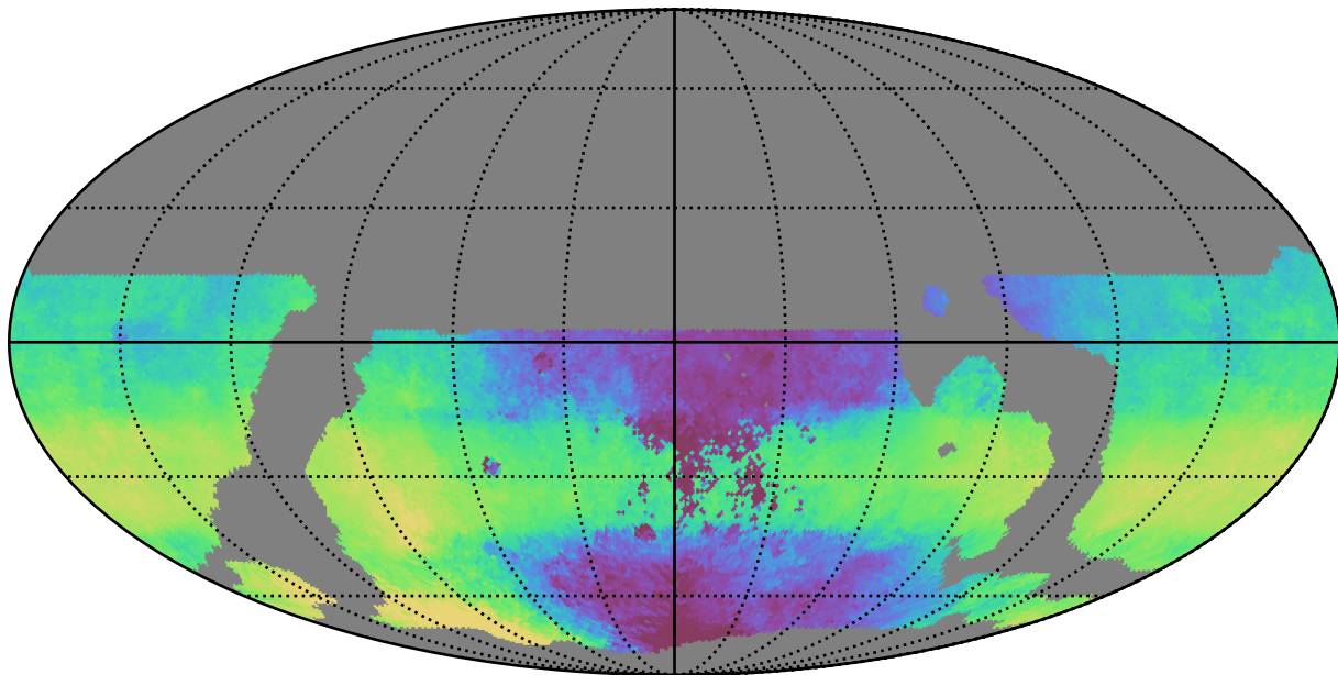
weather_cloudso16v3.4_10yrs WFD y band: Median HA
