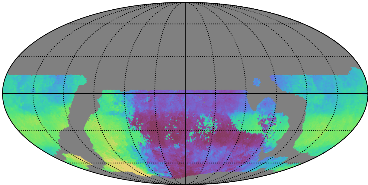
weather_cloudso16v3.4_10yrs WFD u band: Median HA
