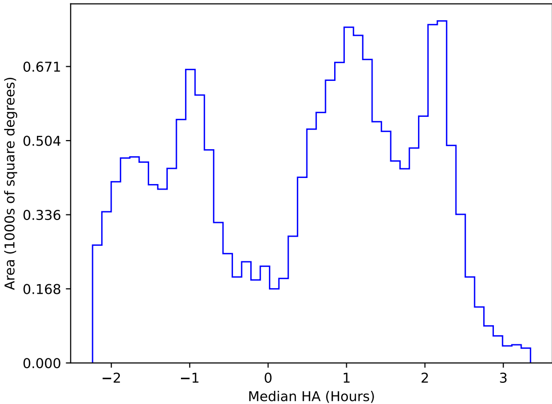
weather_cloudso16v3.4_10yrs WFD u band: Median HA
