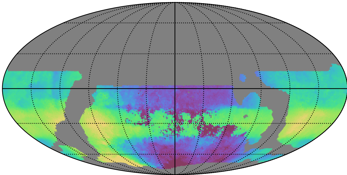
weather_cloudso16v3.4_10yrs WFD r band: Median HA
