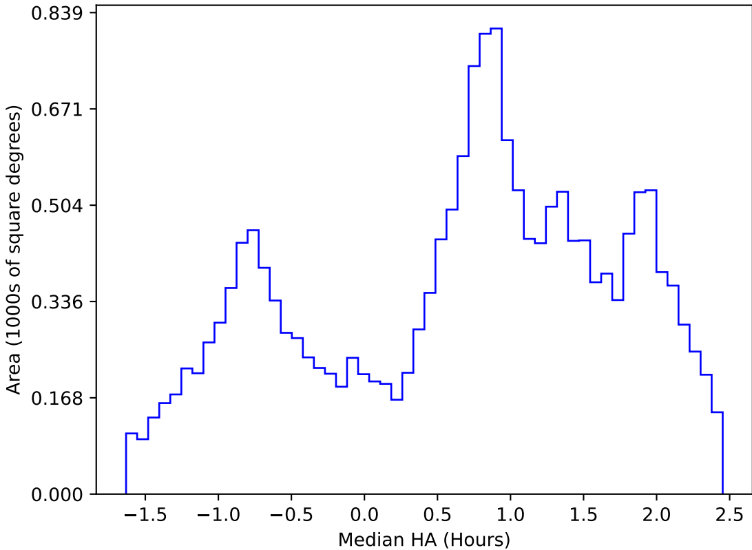
weather_cloudso16v3.4_10yrs WFD r band: Median HA
