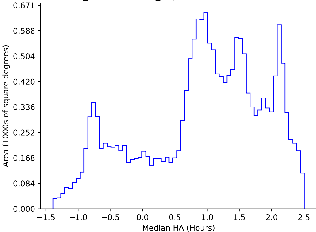
weather_cloudso16v3.4_10yrs WFD all bands: Median HA
