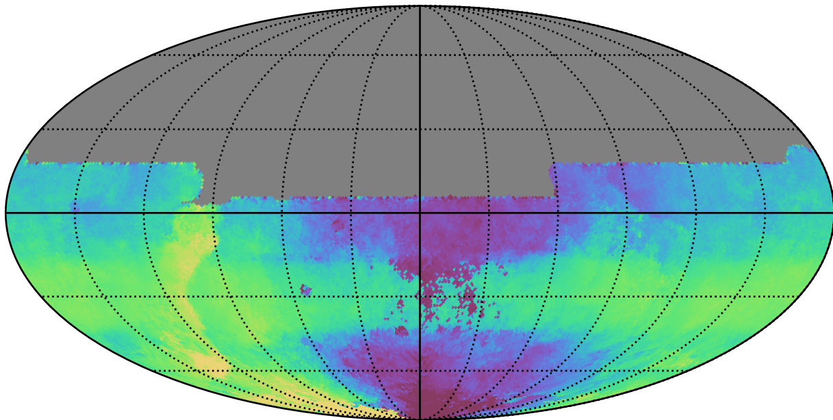
weather_cloudso16v3.4_10yrs All sky y band: Median HA
