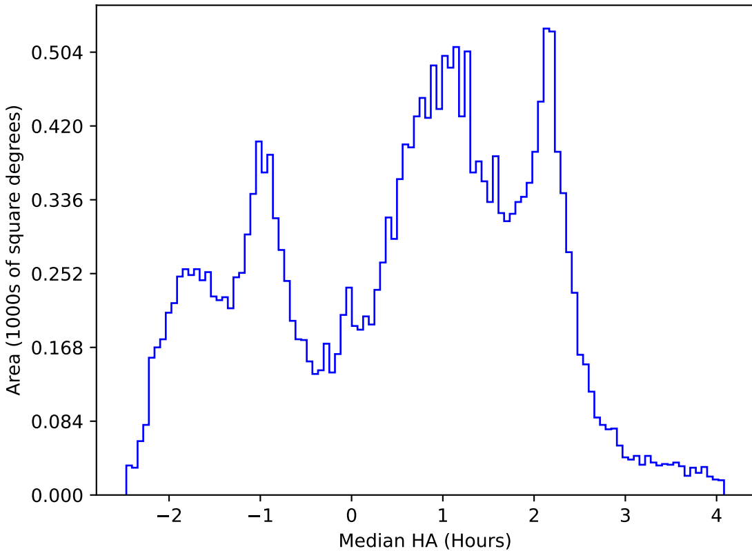
weather_cloudso16v3.4_10yrs All sky u band: Median HA
