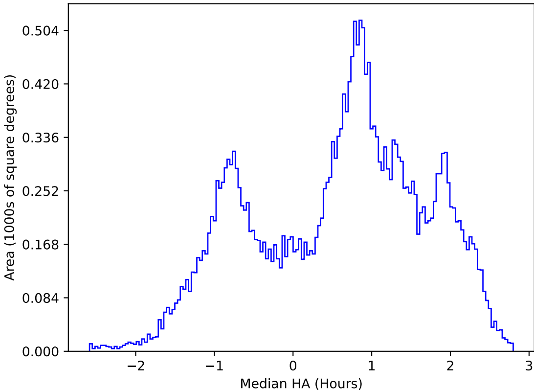
weather_cloudso16v3.4_10yrs All sky r band: Median HA
