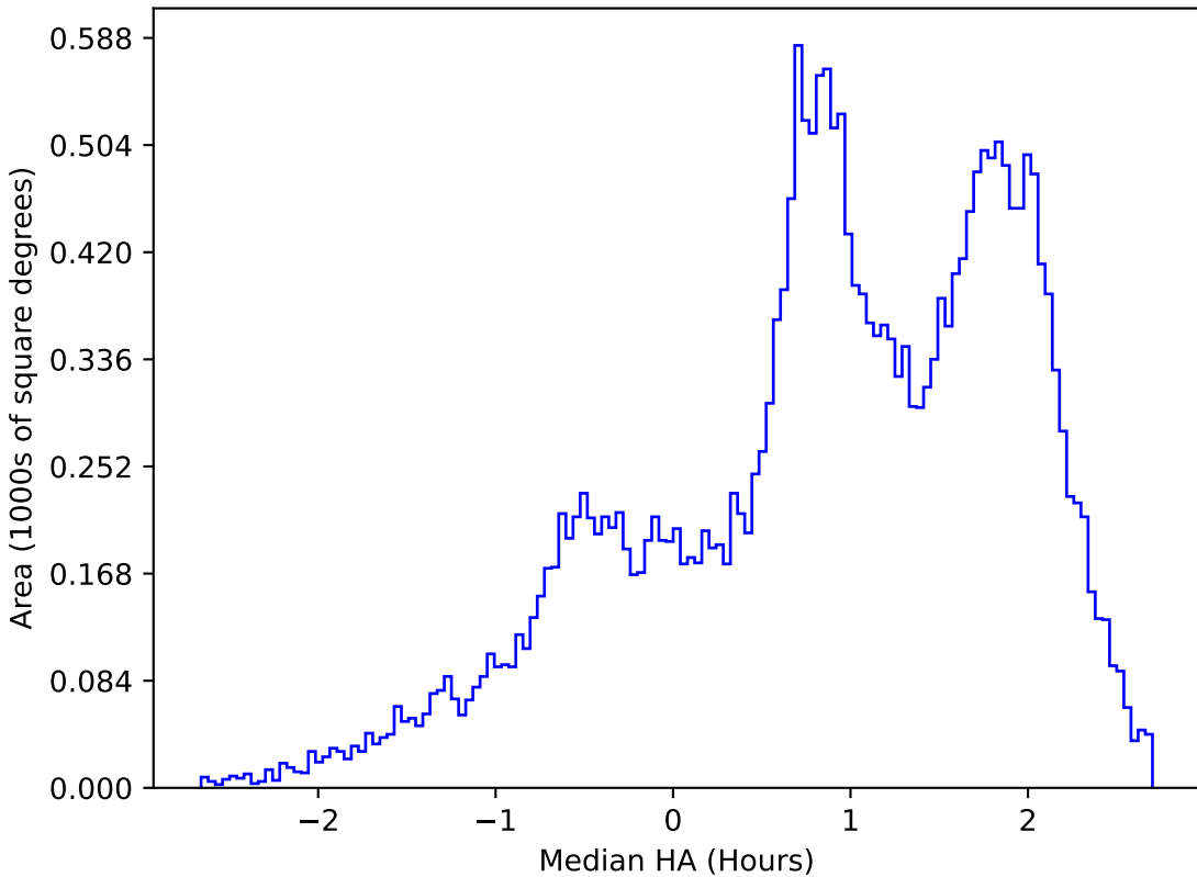
weather_cloudso16v3.4_10yrs All sky i band: Median HA
