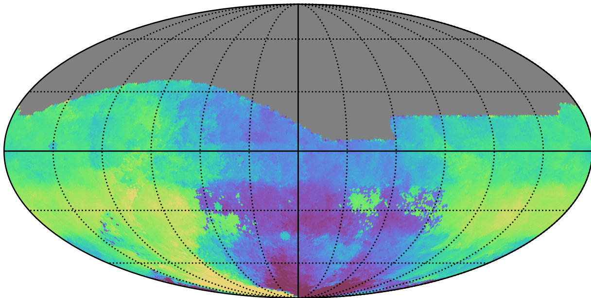
weather_cloudso16v3.4_10yrs All sky g band: Median HA
