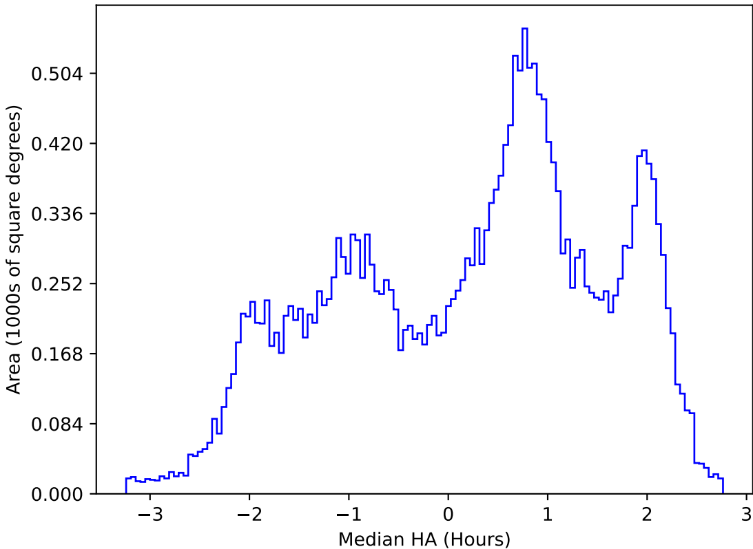
weather_cloudso16v3.4_10yrs All sky g band: Median HA
