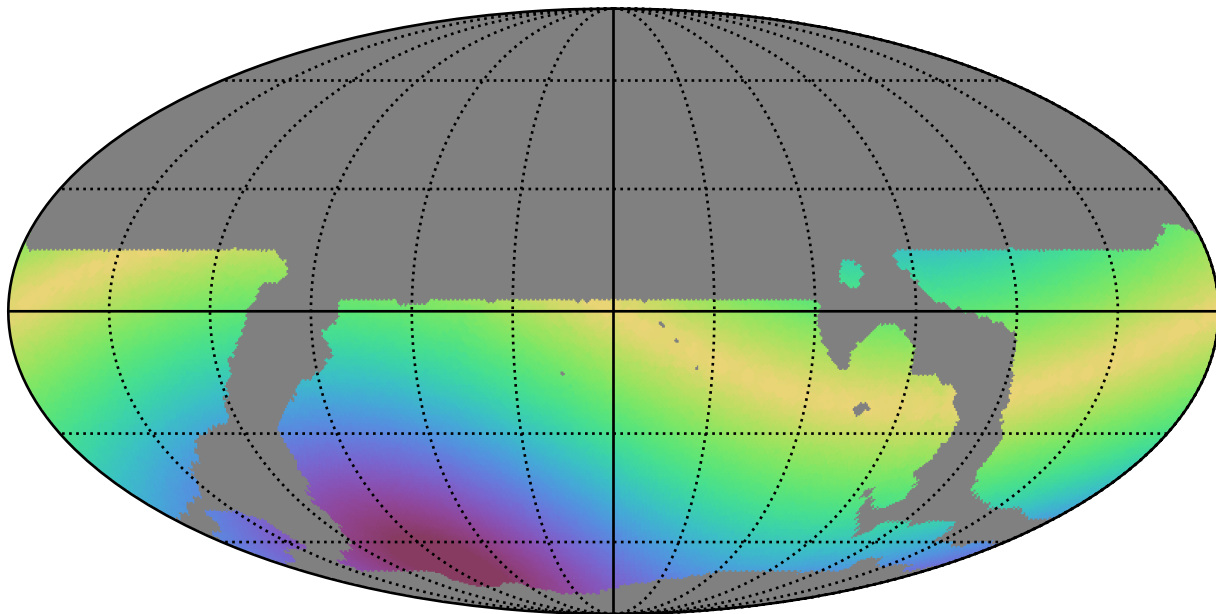
weather_cloudso16v3.4_10yrs WFD r band: Max solarElong
