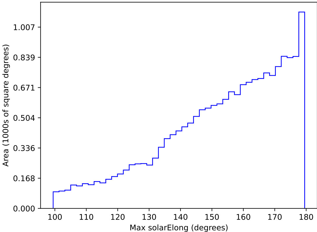
weather_cloudso16v3.4_10yrs WFD r band: Max solarElong
