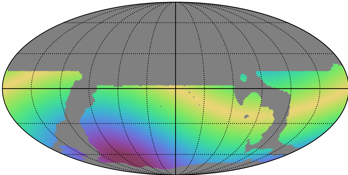
weather_cloudso16v3.4_10yrs WFD all bands: Max solarElong
