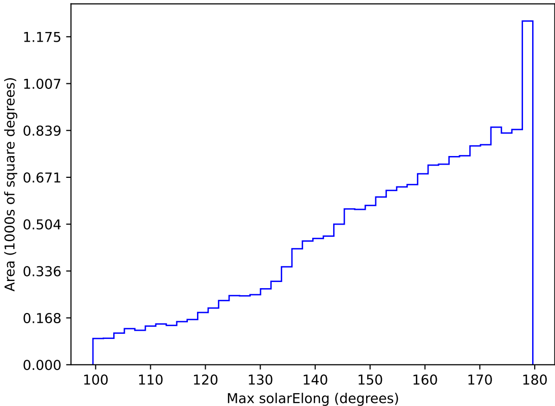
weather_cloudso16v3.4_10yrs WFD all bands: Max solarElong
