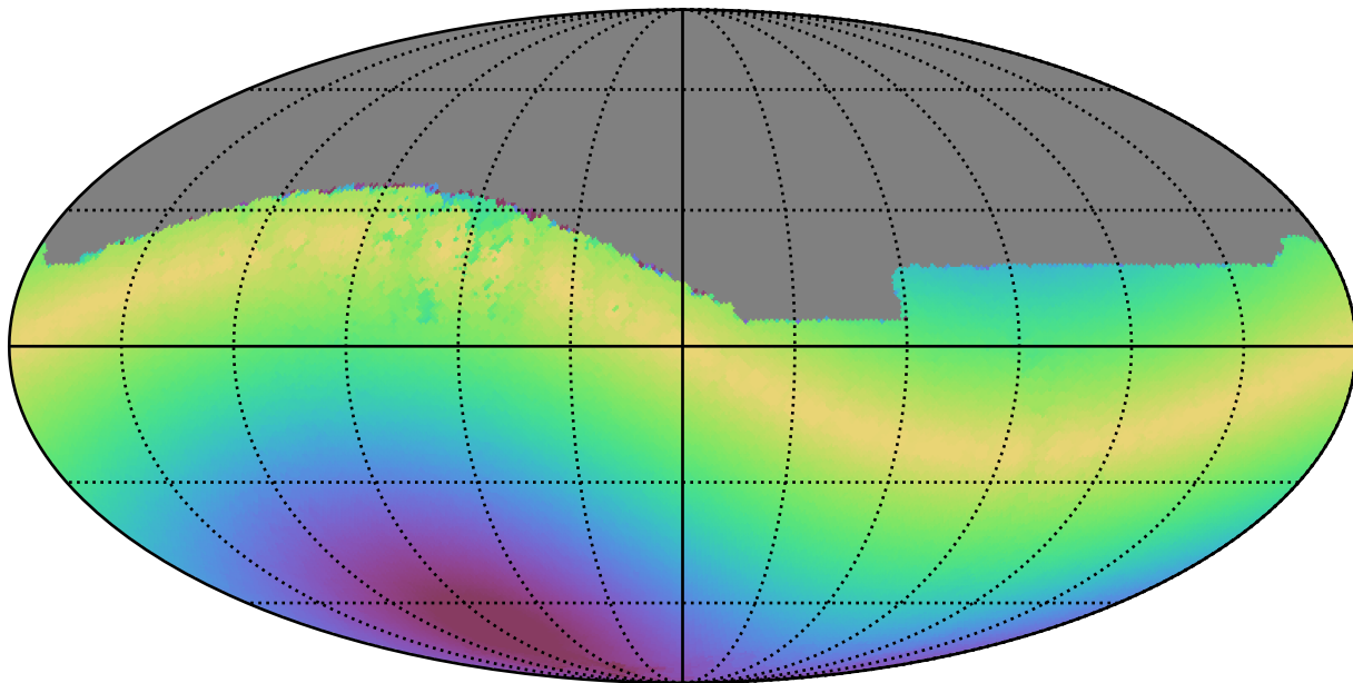
weather_cloudso16v3.4_10yrs All sky z band: Max solarElong
