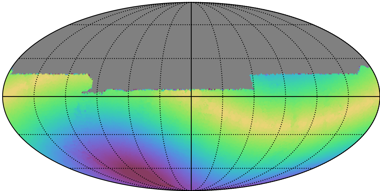
weather_cloudso16v3.4_10yrs All sky u band: Max solarElong
