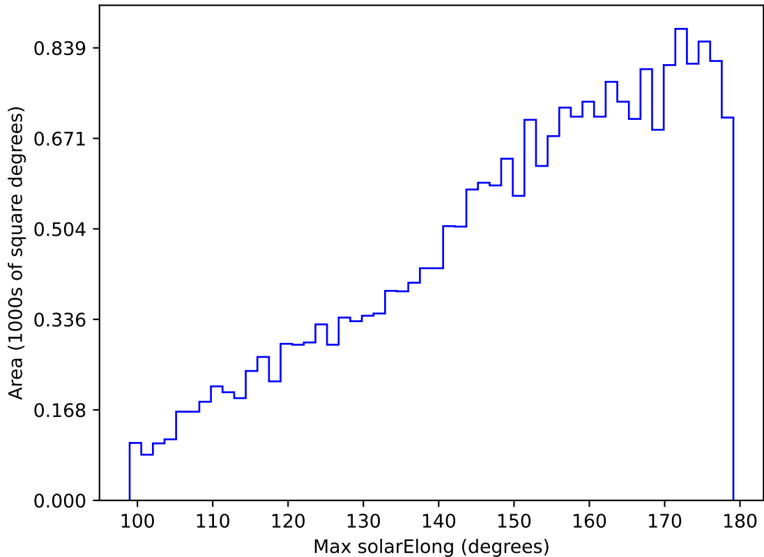
weather_cloudso16v3.4_10yrs All sky u band: Max solarElong
