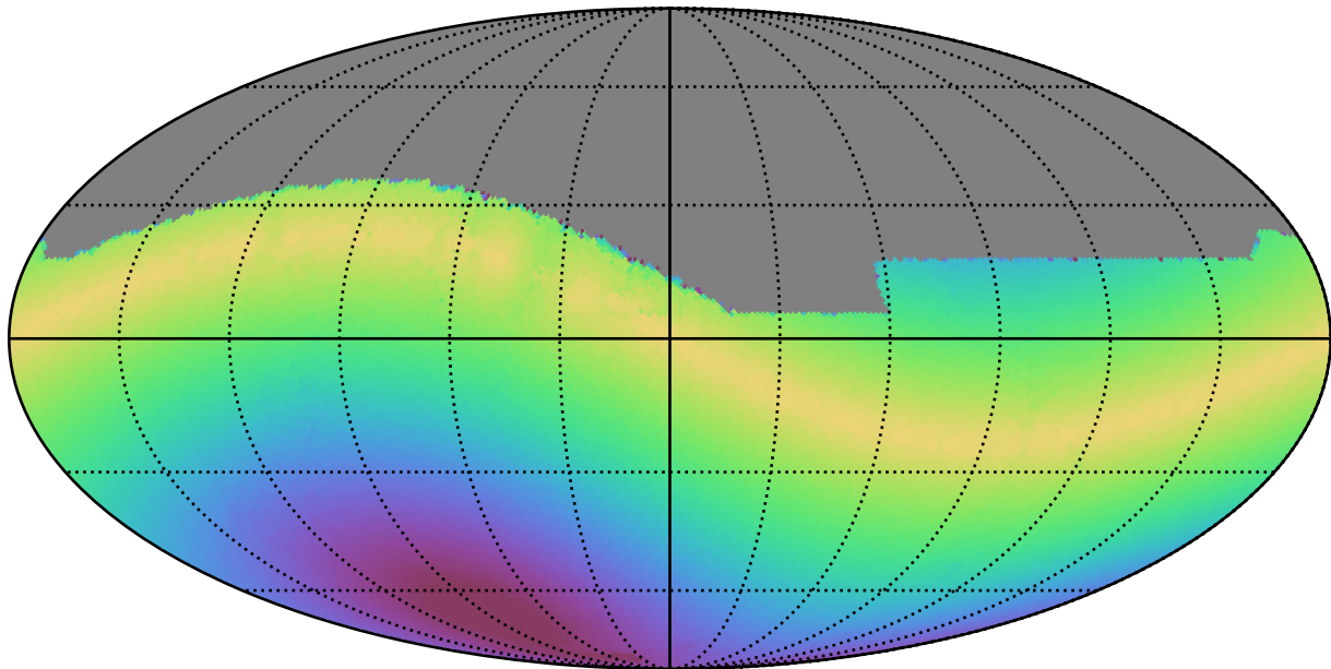
weather_cloudso16v3.4_10yrs All sky r band: Max solarElong
